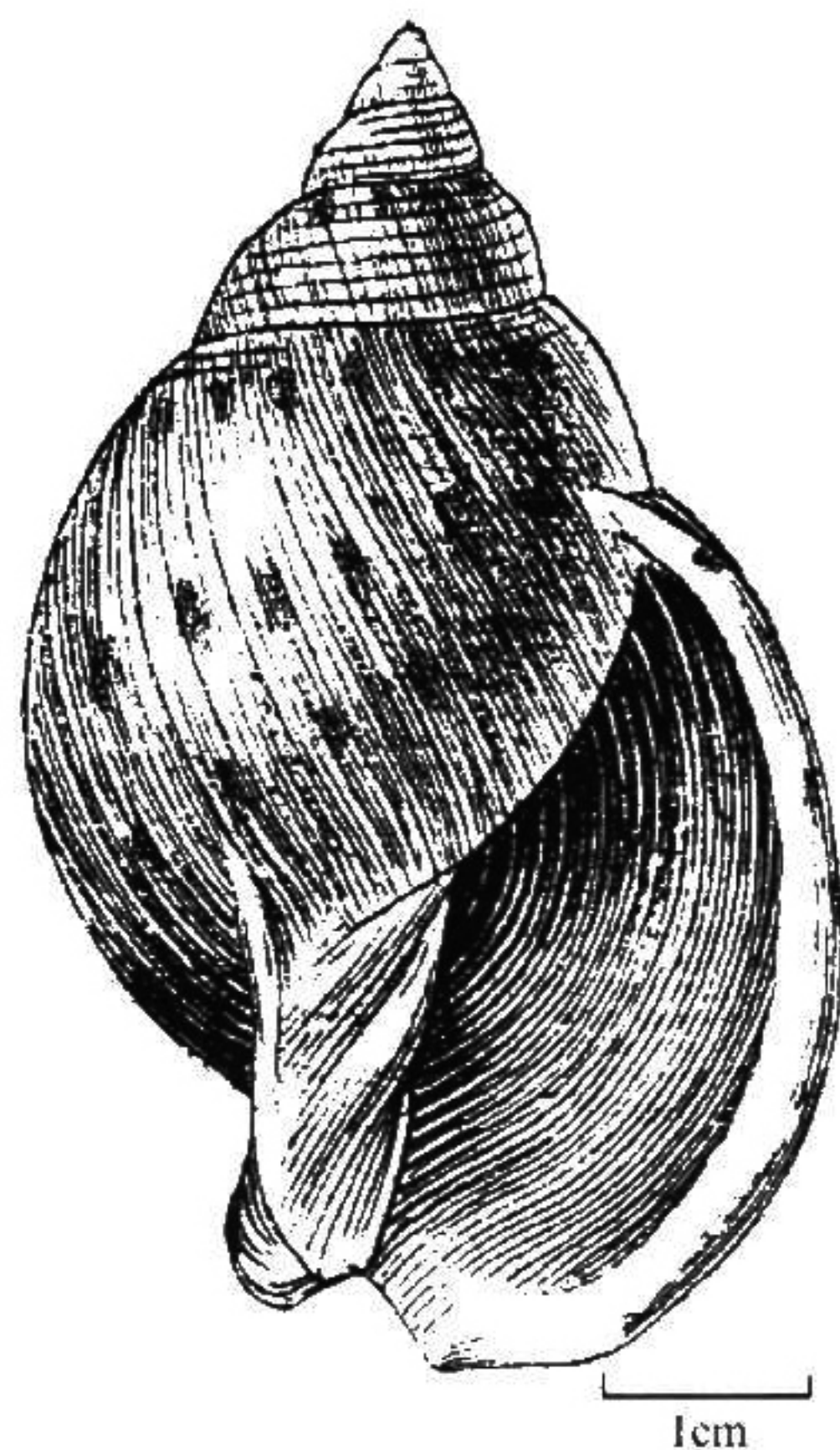
图 31 无饰鬘螺 Phalium (Xenophalium) inornatum (Pilsbry)
